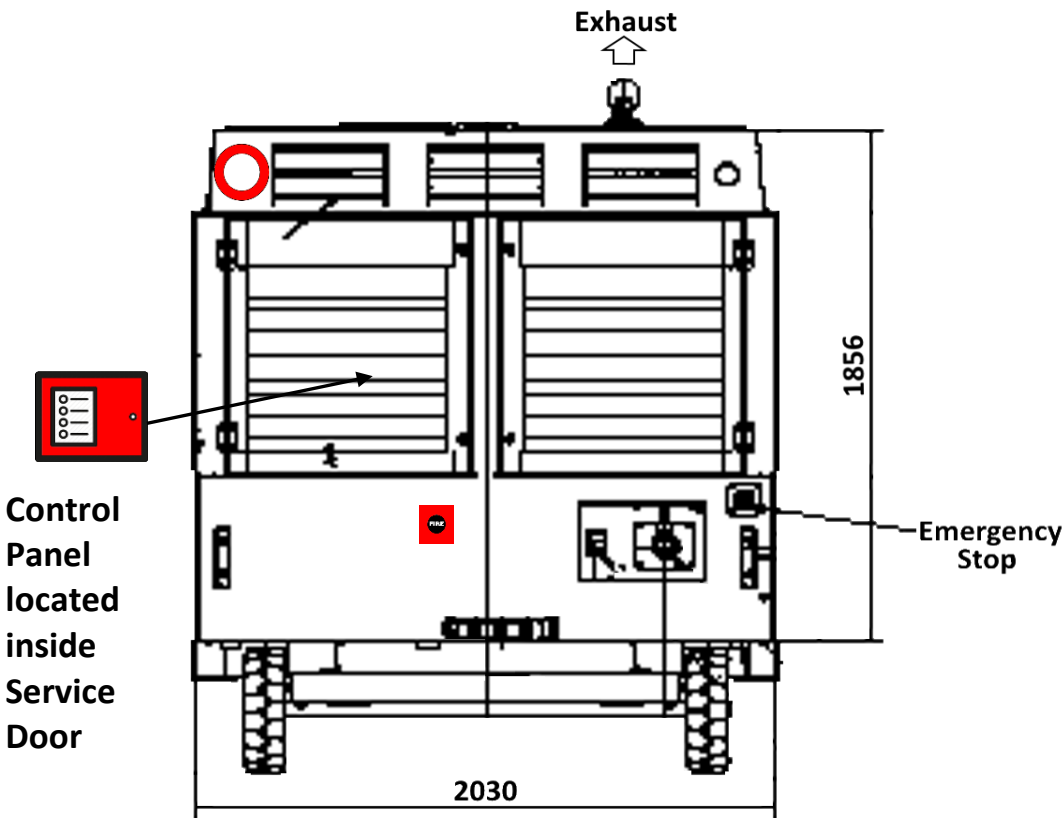
FRONT MOUNTED VIEW
