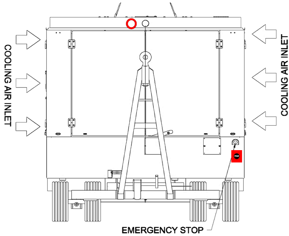
FRONT MOUNTED VIEW
