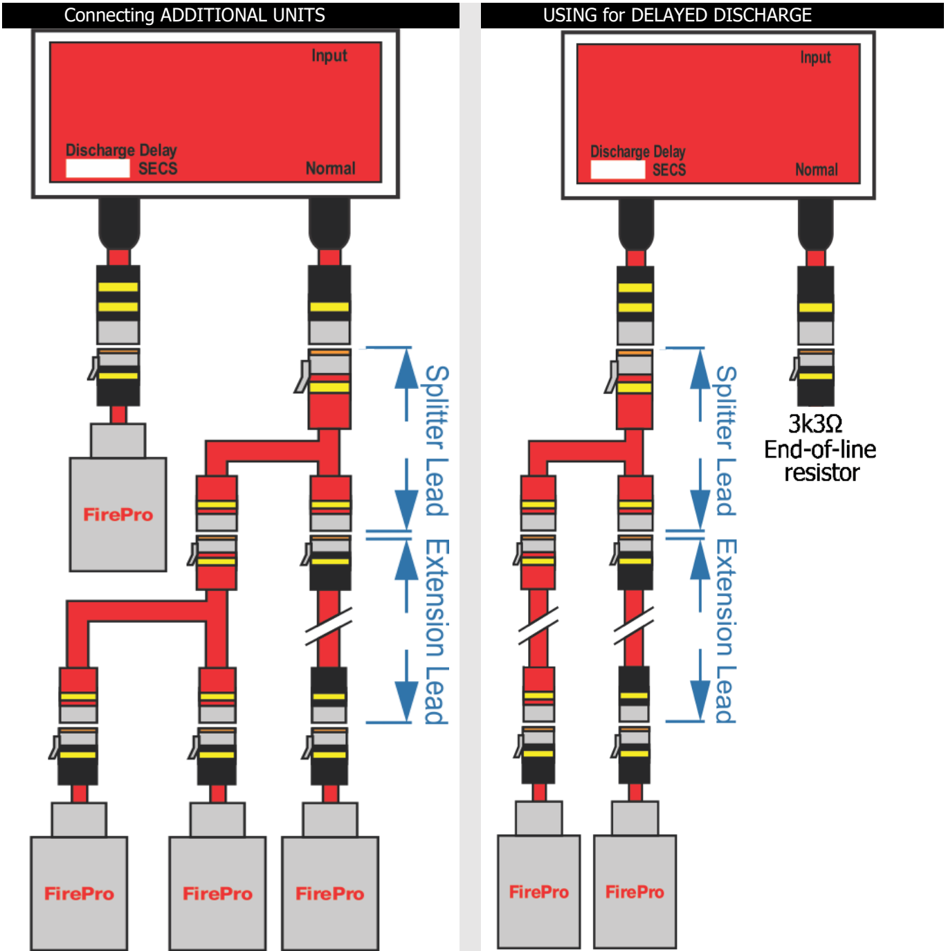
This shows 3 x FirePro Generators operating immediately (through the Normal Activation Circuit) and 1 FirePro unit firing after a delay.
